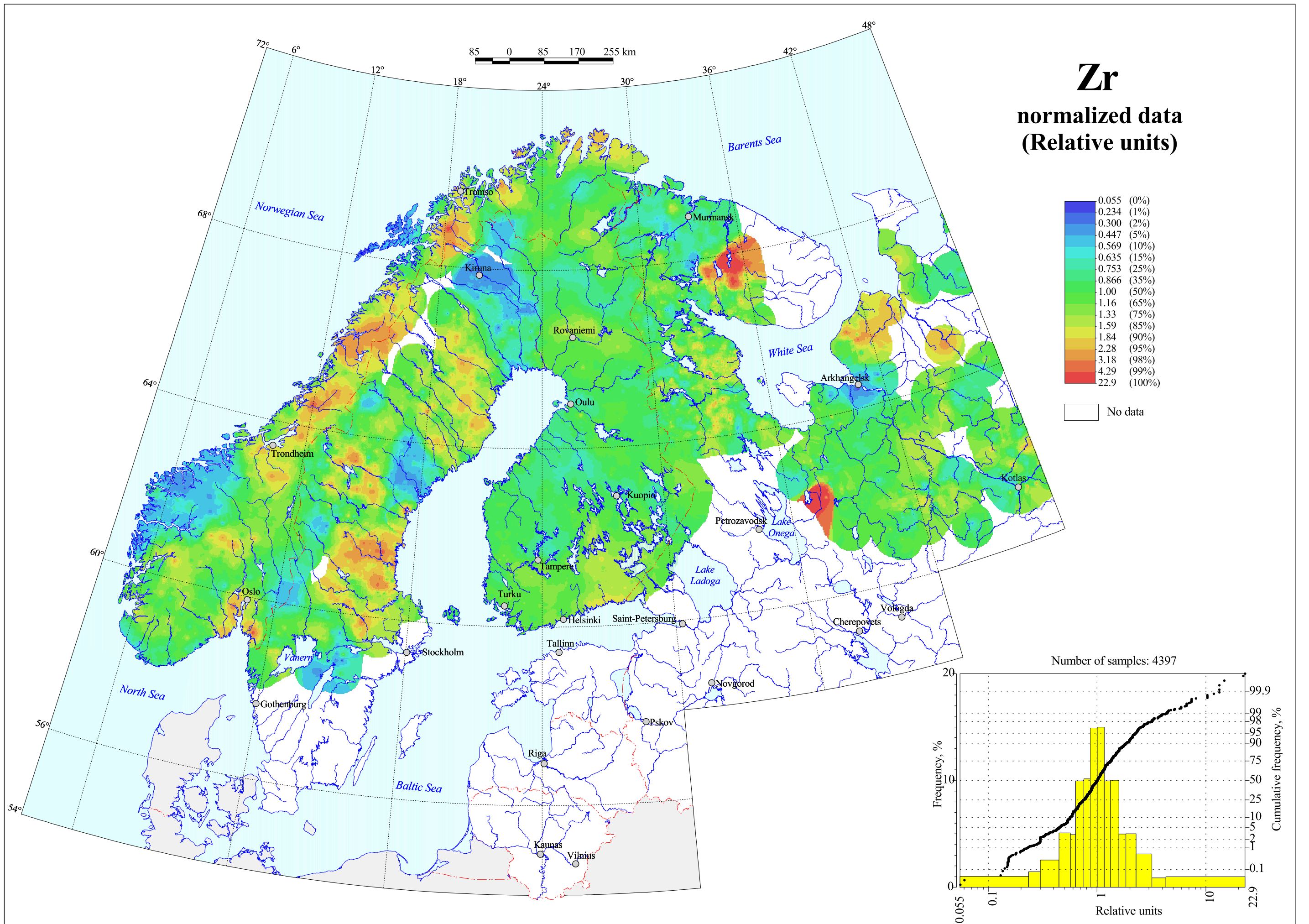
Zirconium in till, grain size <0.06mm
